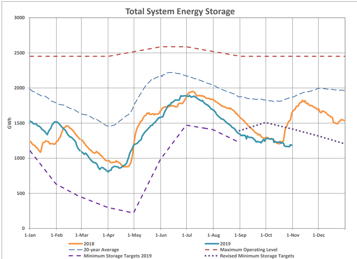
Figure 2: Total System Energy Storage for October 31, 2019
